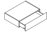
L | W 36 | 14 1/8" 45 | 17 3/4" 54 | 21 1/4" 72 | 28 3/8" 90 | 35 3/8" 108 | 42 1/2" 126 | 49 5/8"
