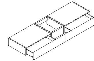
L | W 144 | 15 3/4" 162 | 16 3/4" 180 | 17 7/8" 198 | 18" 216 | 18 5/8"
