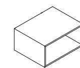
L | W 36 | 14 1/8" 45 | 17 3/4" 54 | 21 1/4" 72 | 28 3/8"
